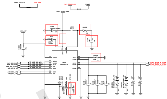
Audio amp
